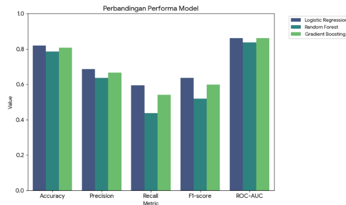
Gambar 5. Perbandingan Performa Model.
